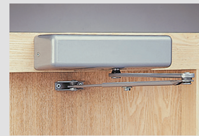
Projecting arm Transom fixing (transom mounted push side)
